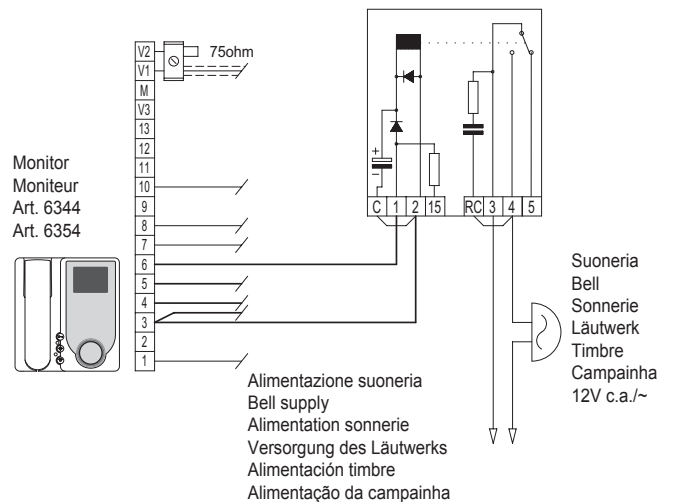
Relè - Relay - Relais Art. 0170/101
