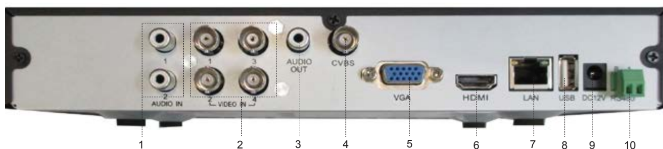
Fig 2-1 Rear Panel for 4-ch
