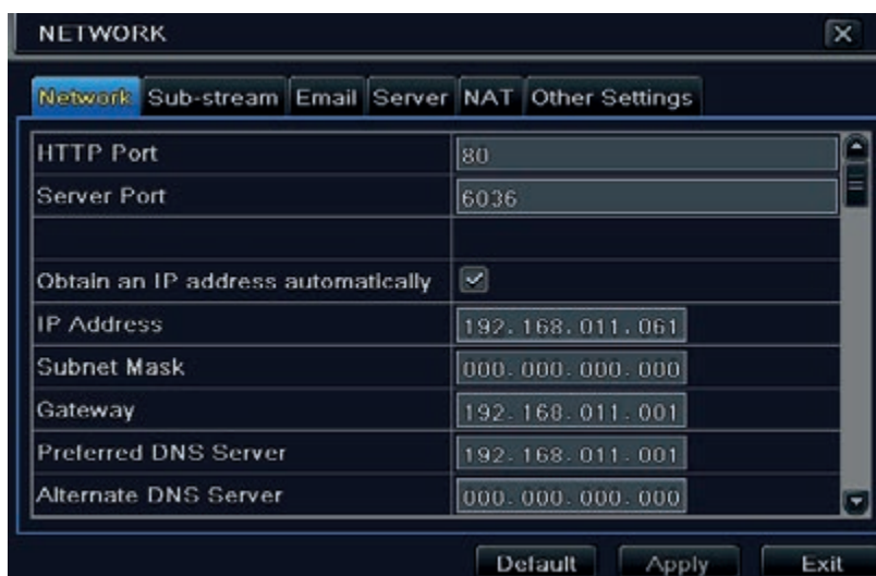
Fig 4-22 Network Configuration-Network
