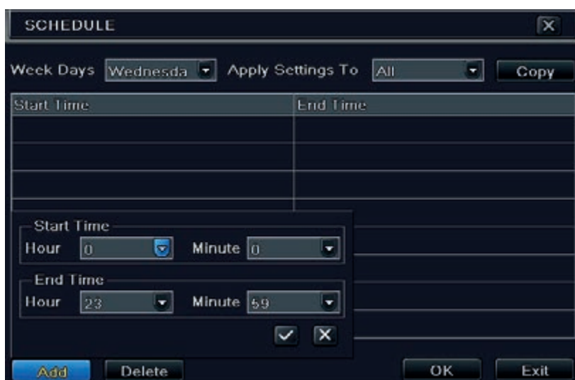
Fig 4-15 Schedule-Week Schedule
