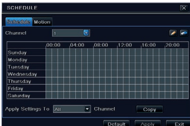
Fig 4-14 Schedule Configuration-Schedule
