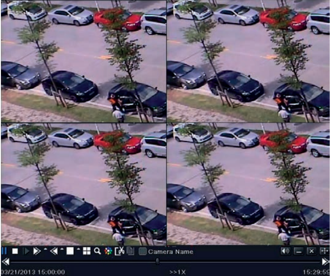
Fig 3-3 Live Playback
