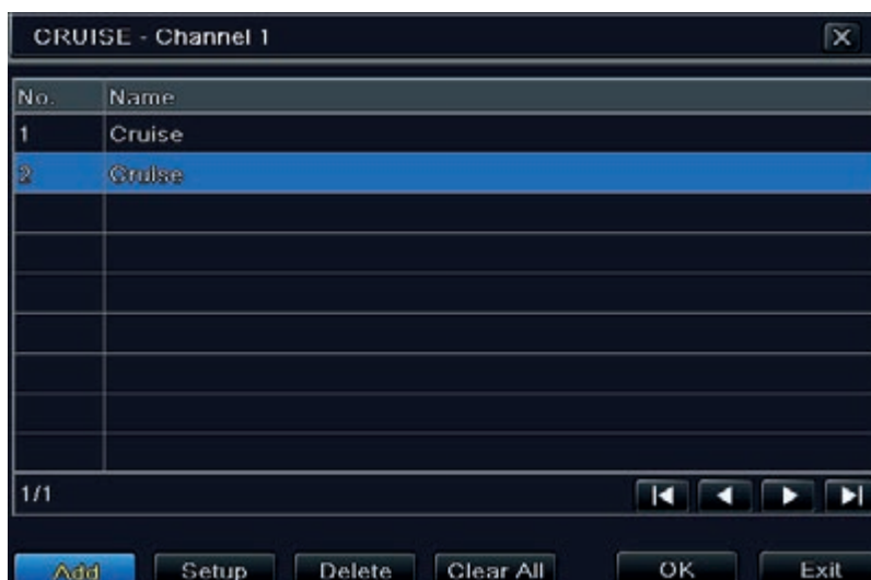
Fig 4-36 Cruise Setting
