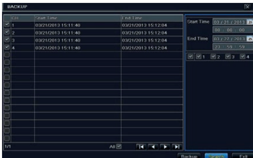
Fig 5-5 Backup Configuration
