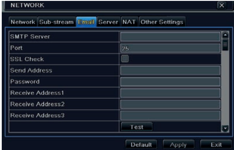
Fig 4-24 Network Configuration-Email
