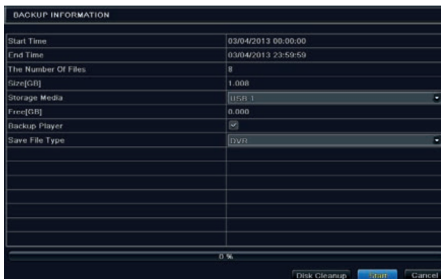
Fig 5-5 Backup Configuration
