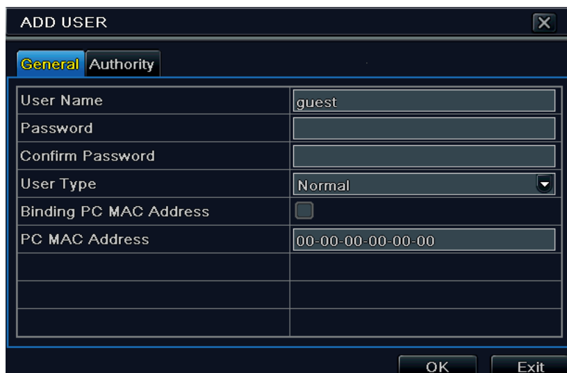
Fig 4-30 Add-General
