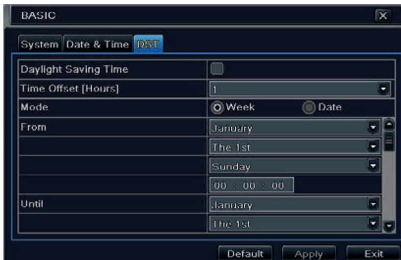
Fig 4-5 Basic Configuration-DST
