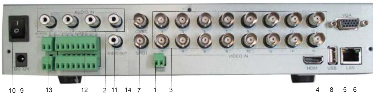
Fig 2-3 Rear Panel for 16-ch
