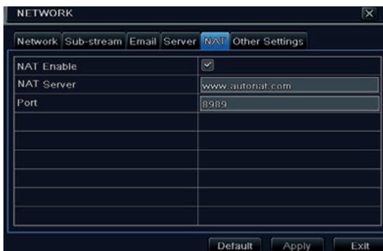
Fig 4-26 Network Configuration-NAT
