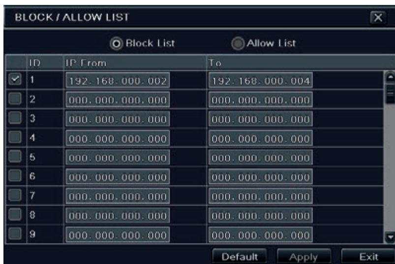
Fig 4-39 Block/Allow List
