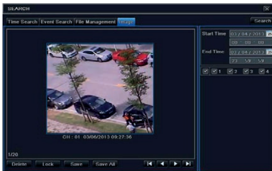
Fig 5-4 Search Configuration-Image
