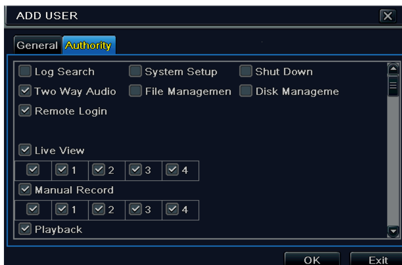
Fig 4-31 Add User-Authority
