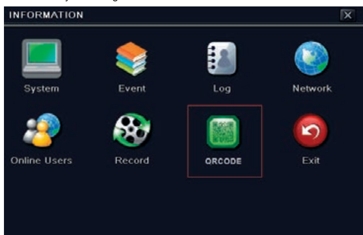
Fig 6-1 Information Configuration
