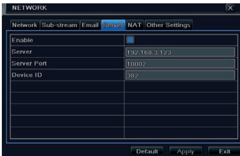
Fig 4-25 Network Configuration-Server
