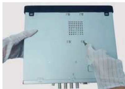
4. Turn over the device and fix the HDD with the screws.
