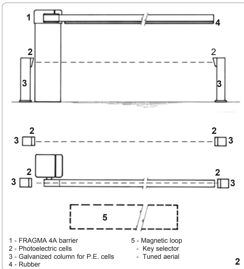
Parts to install meeting the EN 12453 standard
